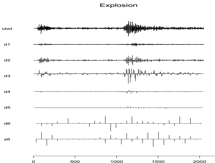
Fig. 4.23. Discrete wavelet transform of the explosion series using the symmlet8 wavelets and J = 6 levels of scale.
