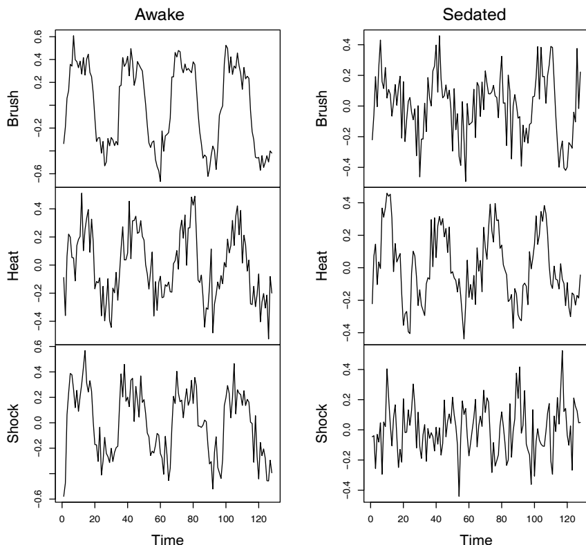
Fig. 7.1. Mean response of subjects to various combinations of periodic stimulæ measured at the cortex (primary somatosensory, contralateral). In the first column, the subjects are awake, in the second column the subjects are under mild anesthesia. In the first row, the stimulus is a brush on the hand, the second row involves the application of heat, and the third row involves a low level shock.
