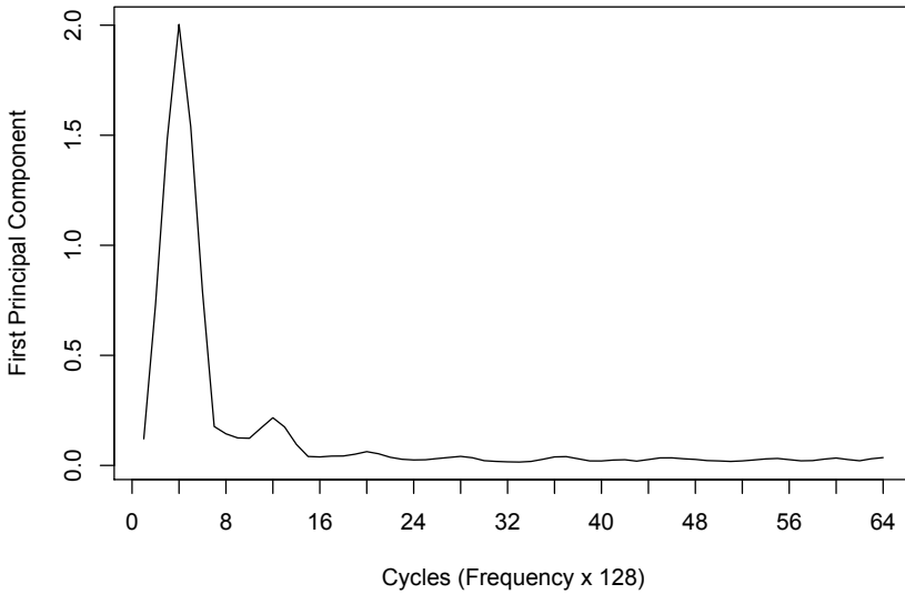
Fig. 7.18. The estimated spectral density, \hat{\lambda}_1(j/128) , of the first principal component series in Example 7.14.
