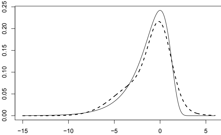
Fig. 6.12. Density of the log of a \chi_1^2 as given by (6.174) (solid line) and the fitted normal mixture (dashed line) from the NYSE example.
